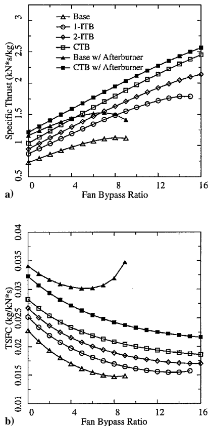
Fig. 8 Performances of turbofan engines vs fan bypass ratio at M_\infty = 0.87 , T_{04} = 1500 K, T_{06} = 1900 K, \pi_c = 40 , and \pi_f = 1.65 .
