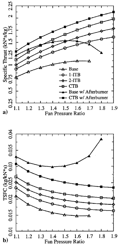
Fig. 9 Performances of turbofan engines vs fan pressure ratio at M_\infty = 0.87 , T_{04} = 1500 K, T_{06} = 1900 K, \pi_c = 40 , and \beta = 8 .
