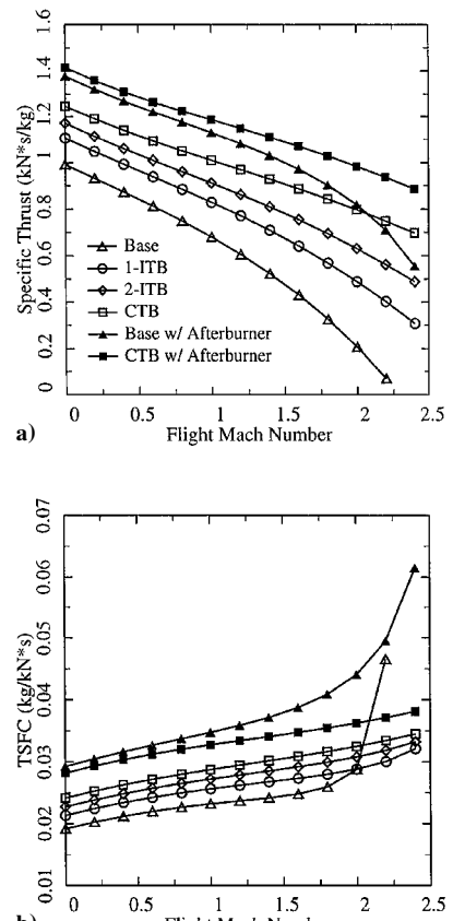
Fig. 10 Performances of turbojet engines vs flight Mach number. T_{04} = 1500 K, T_{06} = 1900 K, and \pi_c = 40 .
