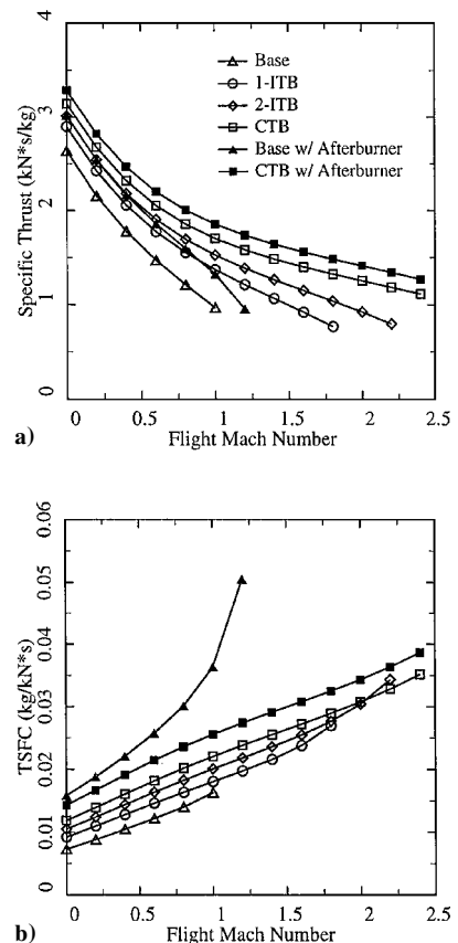
Fig. 11 Performances of turbofan engines vs flight Mach number. T_{04} = 1500 K, T_{06} = 1900 K, \pi_c = 40 , \beta = 8 , and \pi_f = 1.65 .
