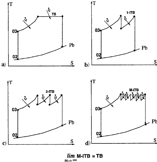
Fig. 3 TB and the M -ITB cycles.
